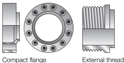
Compact flange
