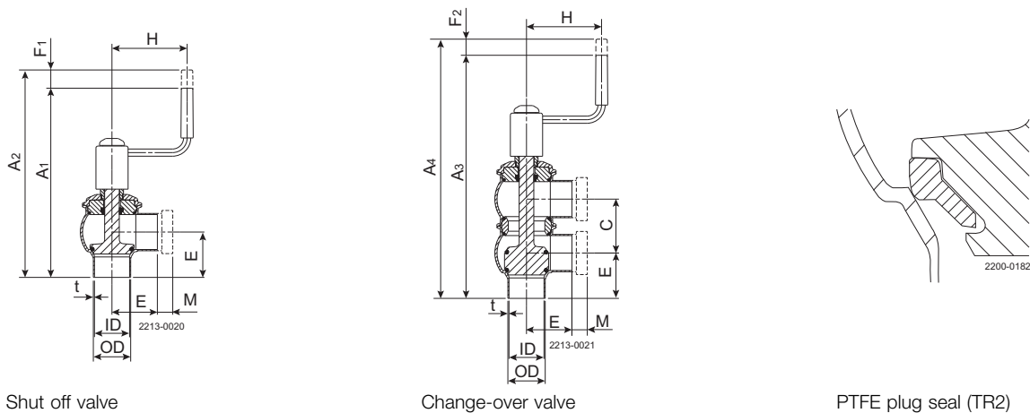
Fig. 2. Dimensions.
